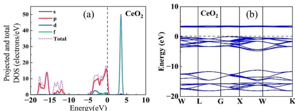
Fig. 2. a): The projected and total density of states (DOSs). b): The band structure of the pristine \text{CeO}_2 at 0 \text{ GPa} .
