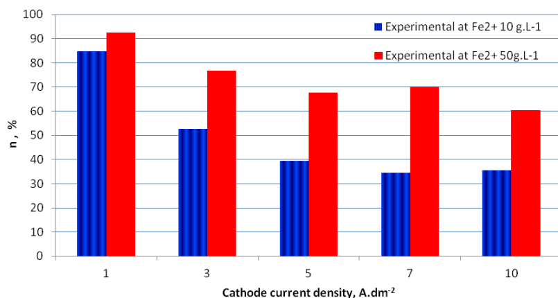
Fig. 6. Current efficiency as a function of applied current density for two \text{Fe}^{2+} concentrations.
