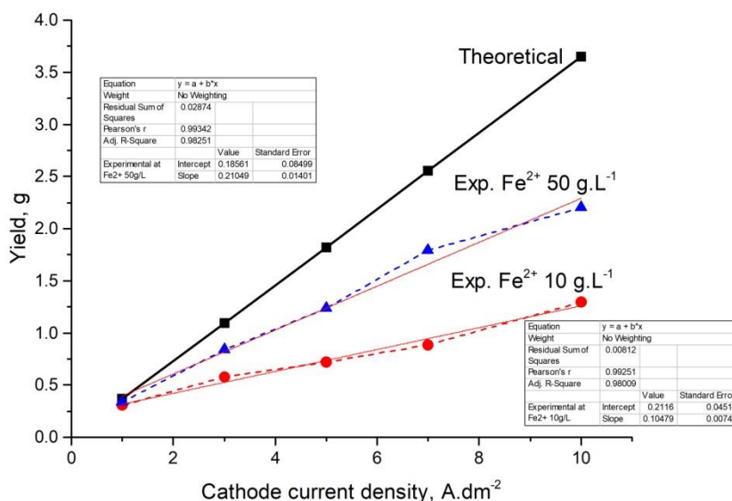
Fig. 7. Comparison between theoretically calculated and experimentally obtained iron powder mass at different current densities for electrolytes containing 10.0 and 50.0 \text{g} \cdot \text{L}^{-1} \text{Fe}^{2+} .
