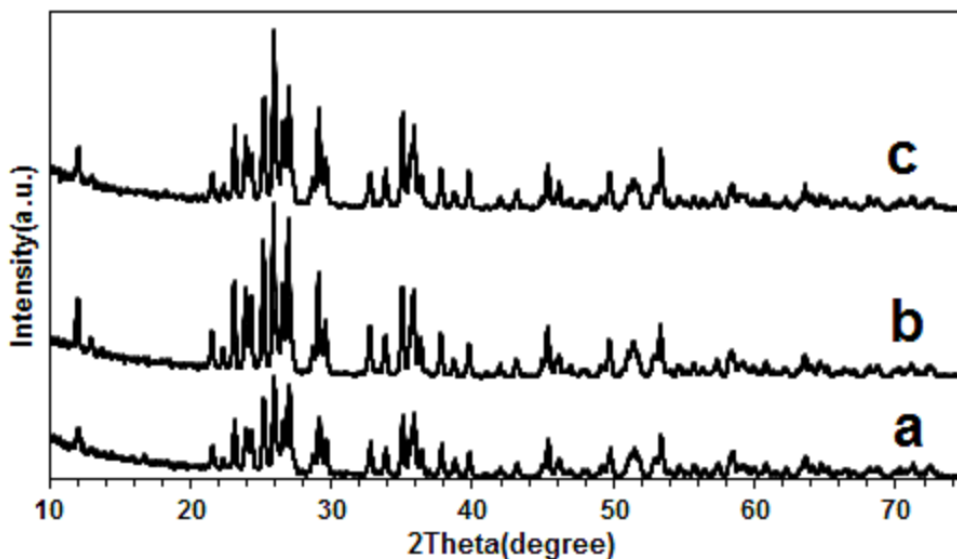
Fig. 4. XRD patterns of the \text{Cu}_3\text{Mo}_2\text{O}_9 samples calcined at 500\text{ }^{\circ}\text{C} with (a) rod, (b) sheet and (c) hollow sphere morphologies.
