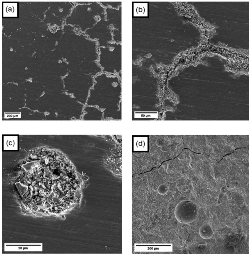
FIGURE 4 The SEM images of sample GP-0
