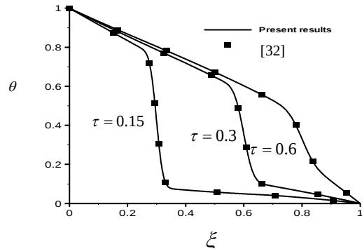
Fig. 2. Thermal distribution inside the slab for several different times
