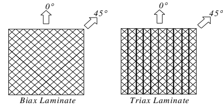
Fig. 3. Two Directions of Available Equivalent Elastic Modulus
