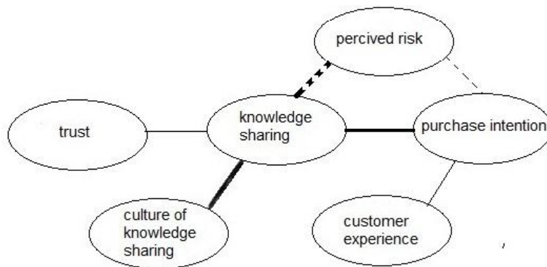
Fig2.final estimated model
