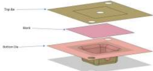
Fig. 2. Shell Elements
