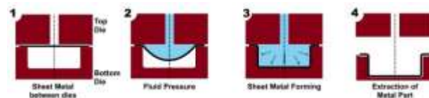
Fig. 1. Sheet Hydroforming
