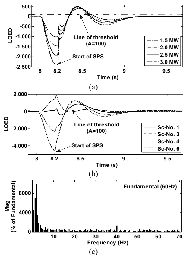
Fig. 8. (a) Calculated LOED of four DFIGs (1.5, 2, 2.5 and 3 MW) at loading No. 14. (b) Calculated LOED of a 1.5 MW DFIG at light and heavy loading scenarios 1, 3, 4 and 6 during SPS. (c) FFT coefficients of the output active power for a 1.5 MW DFIG at loading No. 14 during SPS condition.
