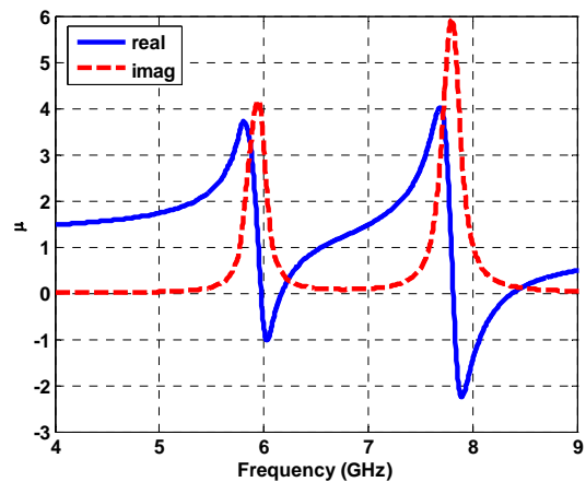
Fig. 6 The retrieved permeability of the proposed structure.
