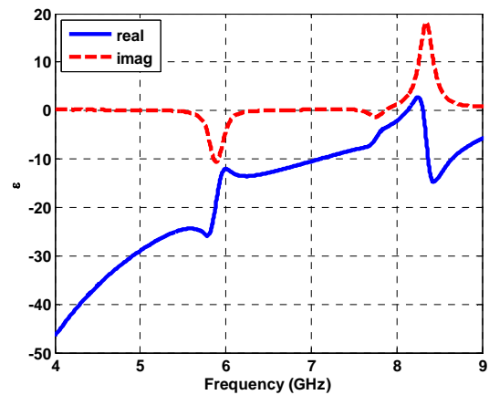
Fig. 5 The retrieved permittivity of the proposed structure.
