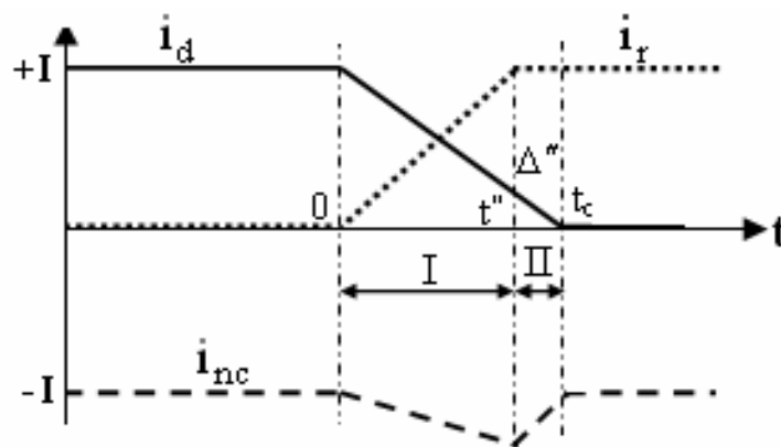
Fig. 3 Current behaviors during commutation.
