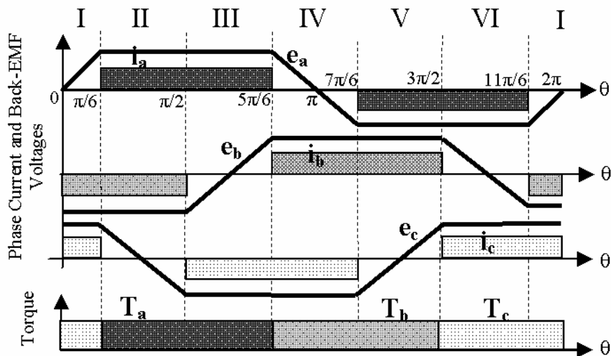
Fig. 1 Ideal signal waveforms of three-phase BLDC motor.
