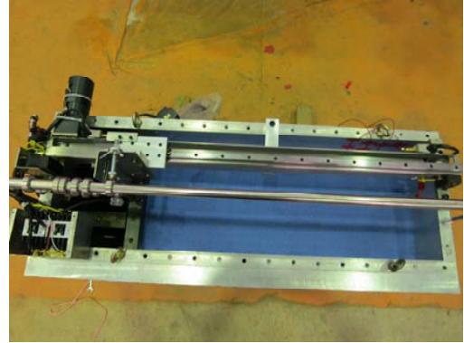
Fig. 2 In-flight surface profile scanner
