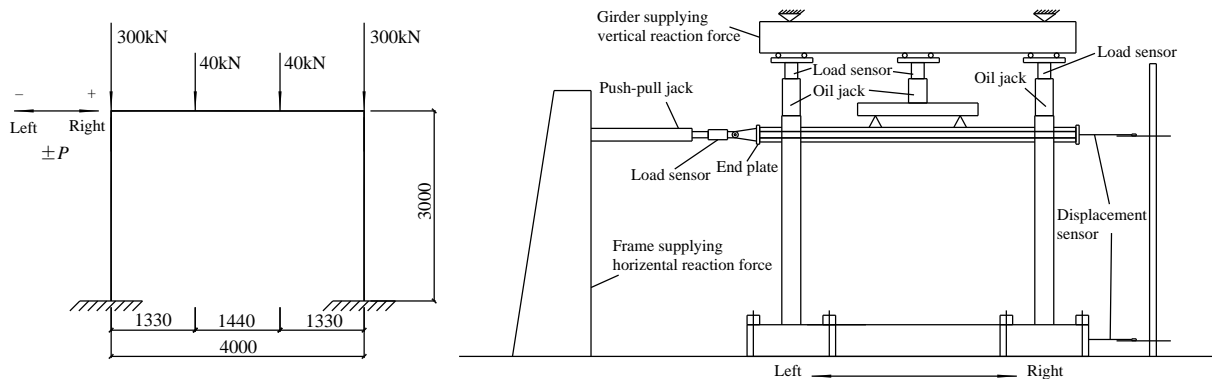
(a) Sketch of loading (b) Loading apparatus Fig. 5 Loading and loading apparatus of specimens
