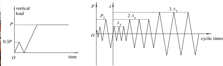
(a) Vertical loading (b) Horizontal loading Fig. 7 Loading rule in tests
