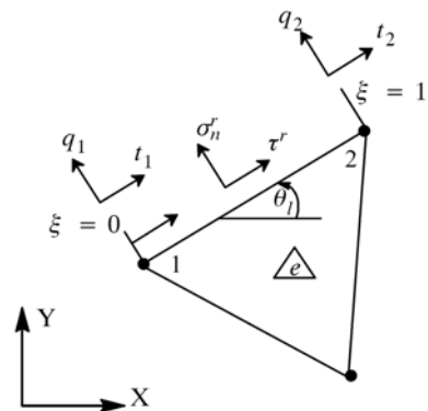
Fig. 3. Stress boundary conditions and external stresses acting on free boundary of element c [11]
