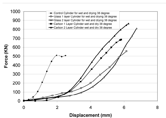
Fig. 8. Load-Deflection curve for group II specimens
