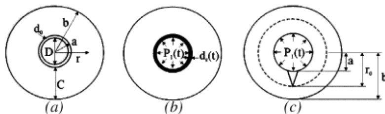
Fig. 1. Schematic representation of cracking process[24]
