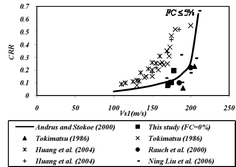
Fig. 15. Comparison between converted CRR field - V_{s1} data based on the laboratory data from clean sand ( FC \leq 5\% ) and the existing field-based correlation of Andrus and Stokoe [1]
