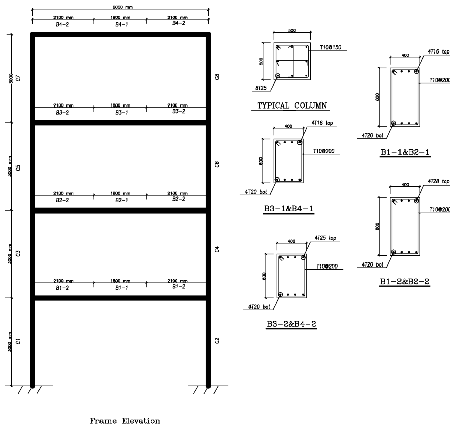
Fig. 11. Geometry and configuration of 4-story frame
