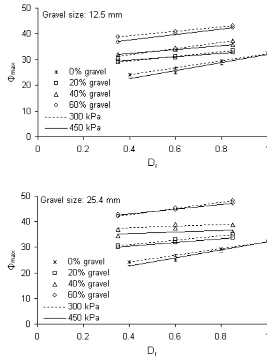
Fig.12 Effect of surcharge pressure and relevant particle crushing on maximum friction angle for different mixtures
