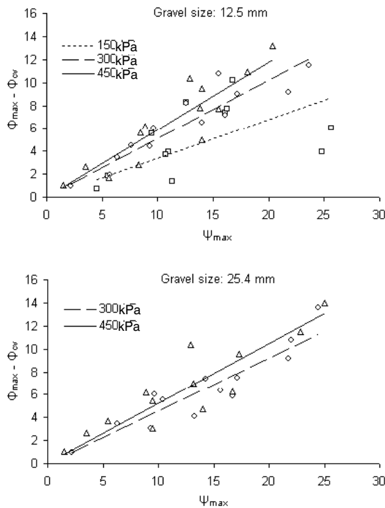
Fig.10 Bolton's [8] equation for sand-gravel mixtures tested under different surcharge pressures
