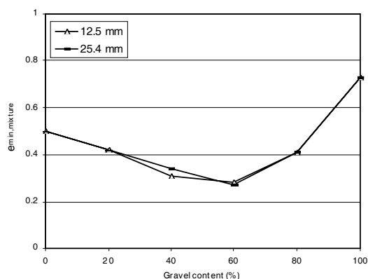
Fig.2 Maximum and minimum void ratios of different mixtures
