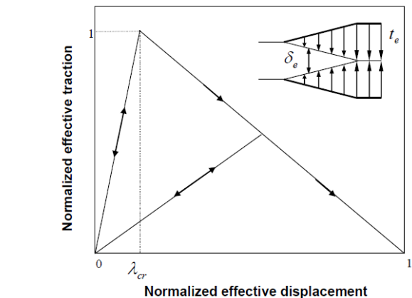
Fig. 2 a bilinear cohesive law in the term of normalized effective displacement and normalized effective traction
