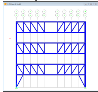
(c) Transverse Frame, Odd Axis (N-S)
