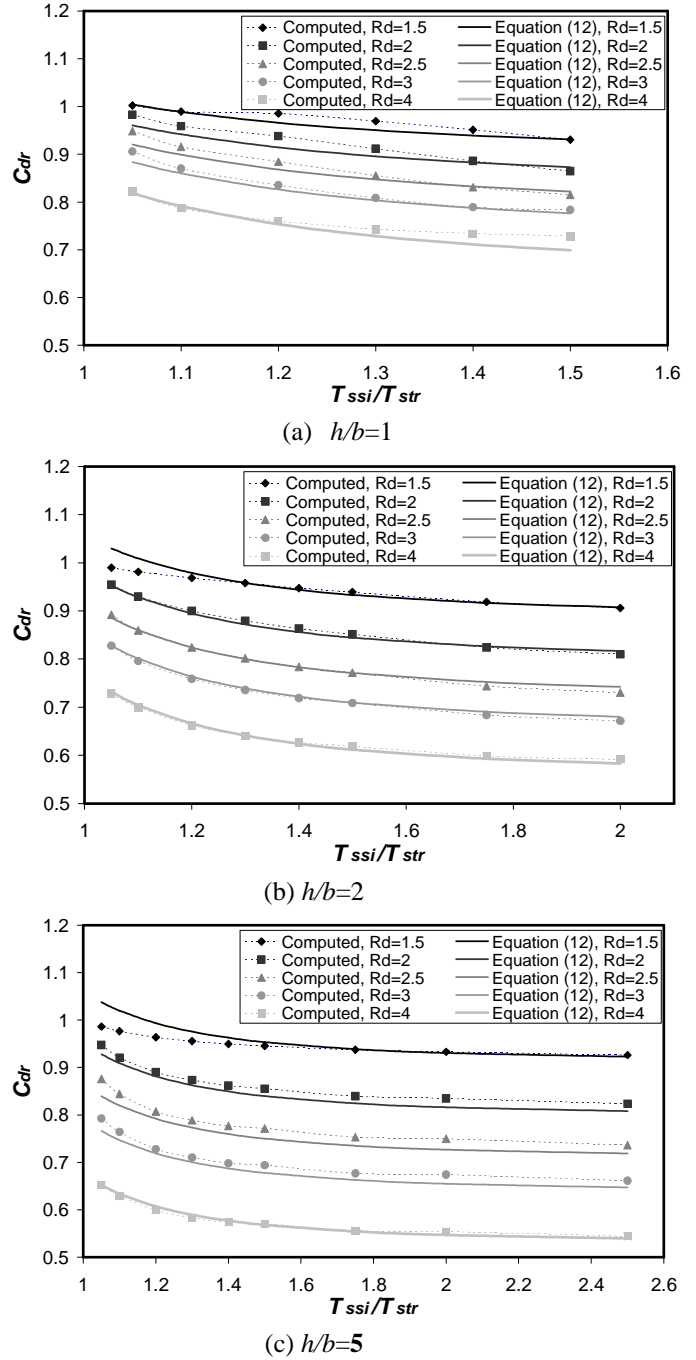
Fig. 12 Comparison of the regressed function of Eq. (12) with the computed exact values for some examples
