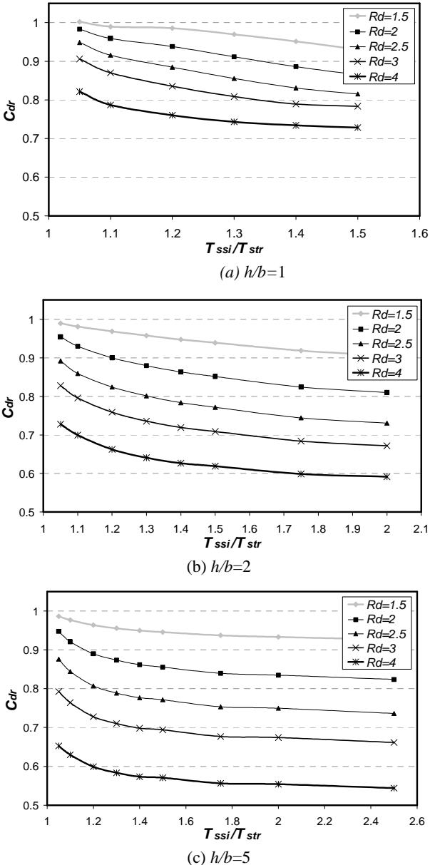
Fig. 11 Mean values of C_{dr} for systems with period larger than 0.5 sec for all site classes
