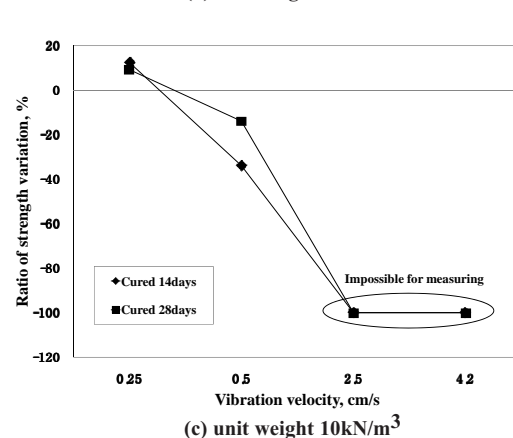
Fig. 8 Comparison of strength variation to curing days of T0 specimens
