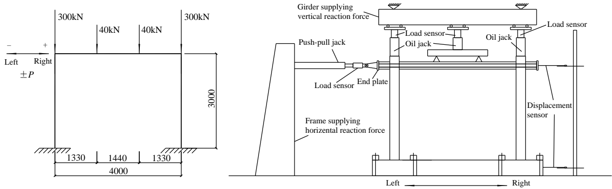
(a) Sketch of loading
