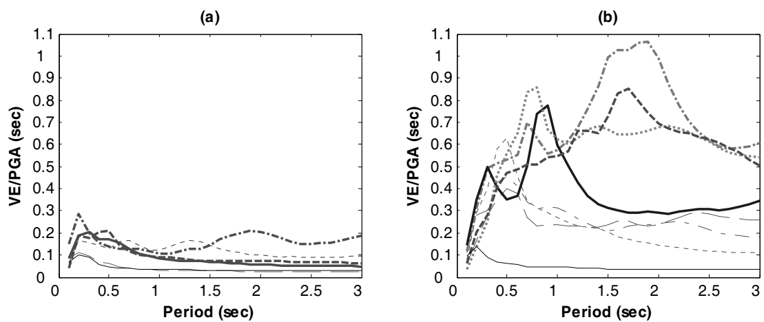
Fig.4 Input energy spectra of the ground motions recorded in ground type 4 (a) for duration \geq 10 sec (b) for duration > 10 sec
