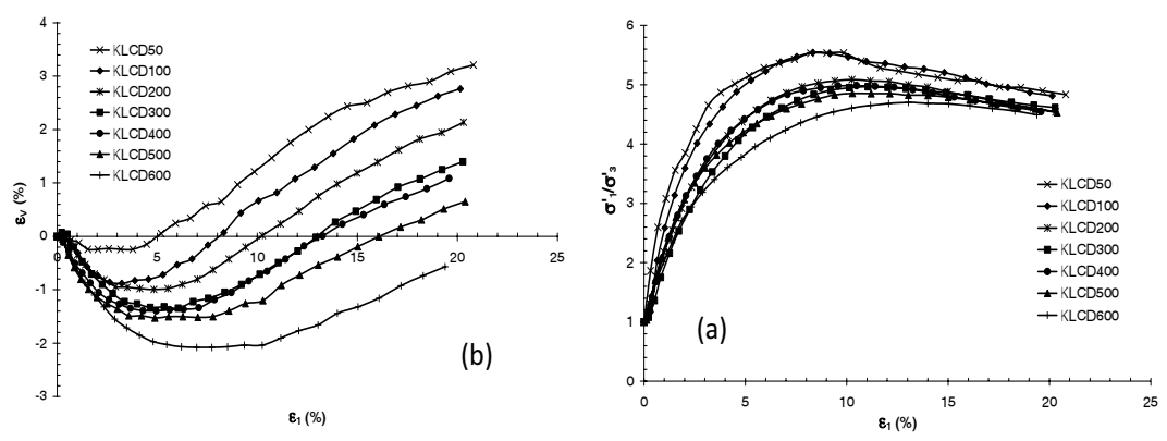
Fig. 3 Triaxial test results on Kish Island sand in loose state (a) \sigma'_1/\sigma'_3 (b) volumetric strain against axial strain
