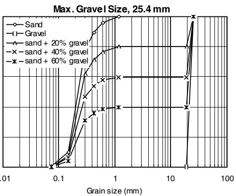
Fig.1 Gradation curves of different sand-gravel mixtures
