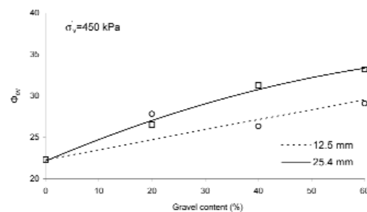
Fig.6 Results of critical state friction angle determination versus gravel fraction for different surcharge pressures
