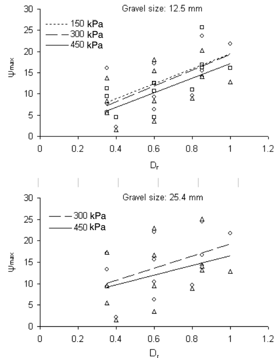
Fig.9 Variation of maximum dilatancy ( \psi_{\max} ) with relative density for different surcharge pressures
