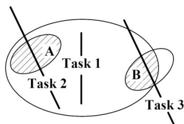
Fig. 2. Task "Closeness".
