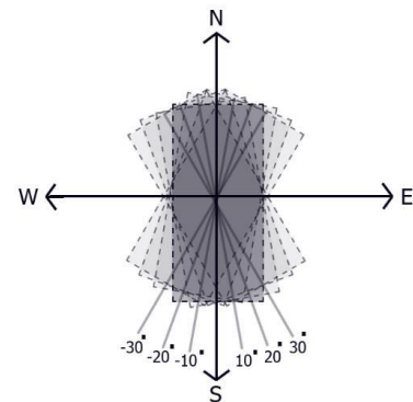
Fig 3. Seven Orientations of the Land Plot in the Simulation
