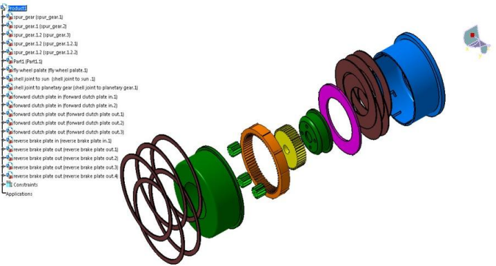
Fig5.planetary gearbox components at second mechanism
