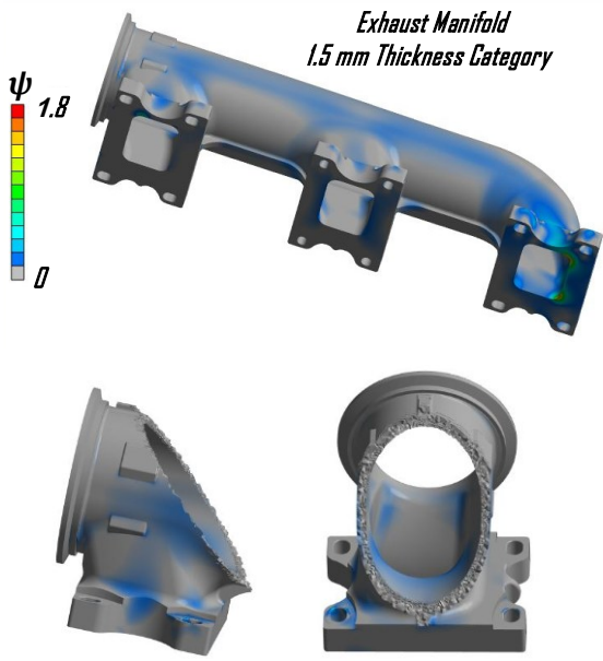
Figure 11: Non-dimensional stress ( \psi ) in the nonconformal part (minimum outlet thickness 1.5 mm)
