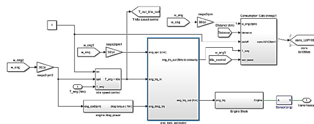
Figure 8: Internal Combustion Engine (ICE) Block Diagram.
