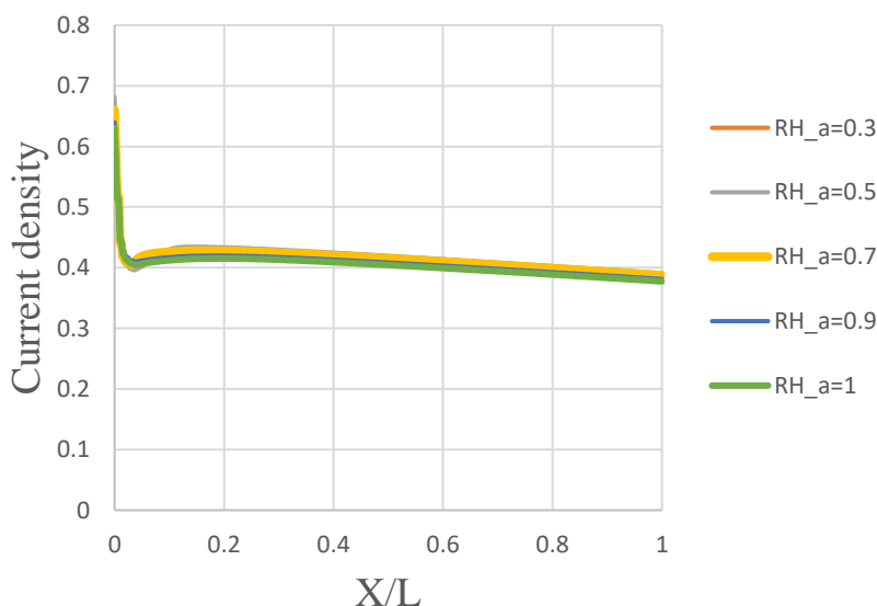
Fig.4. Current density of PEM fuel cell in different relative humidity. (a)Cathode side of PEMFC (b)Anode side of PEMFC
