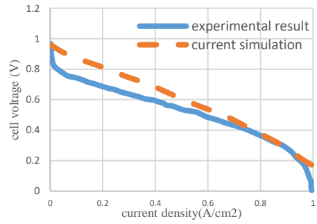
Fig.2. Validation of current simulation with experimental model results [14]
