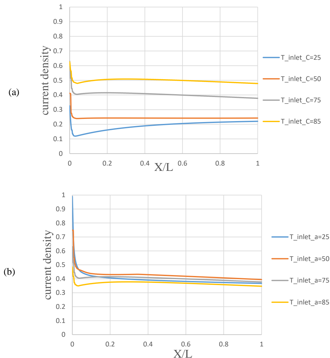
Fig.5. Current density of PEM fuel cell in different inlet temperatures. (a)Cathode side of PEMFC (b) Anode side of PEMFC
