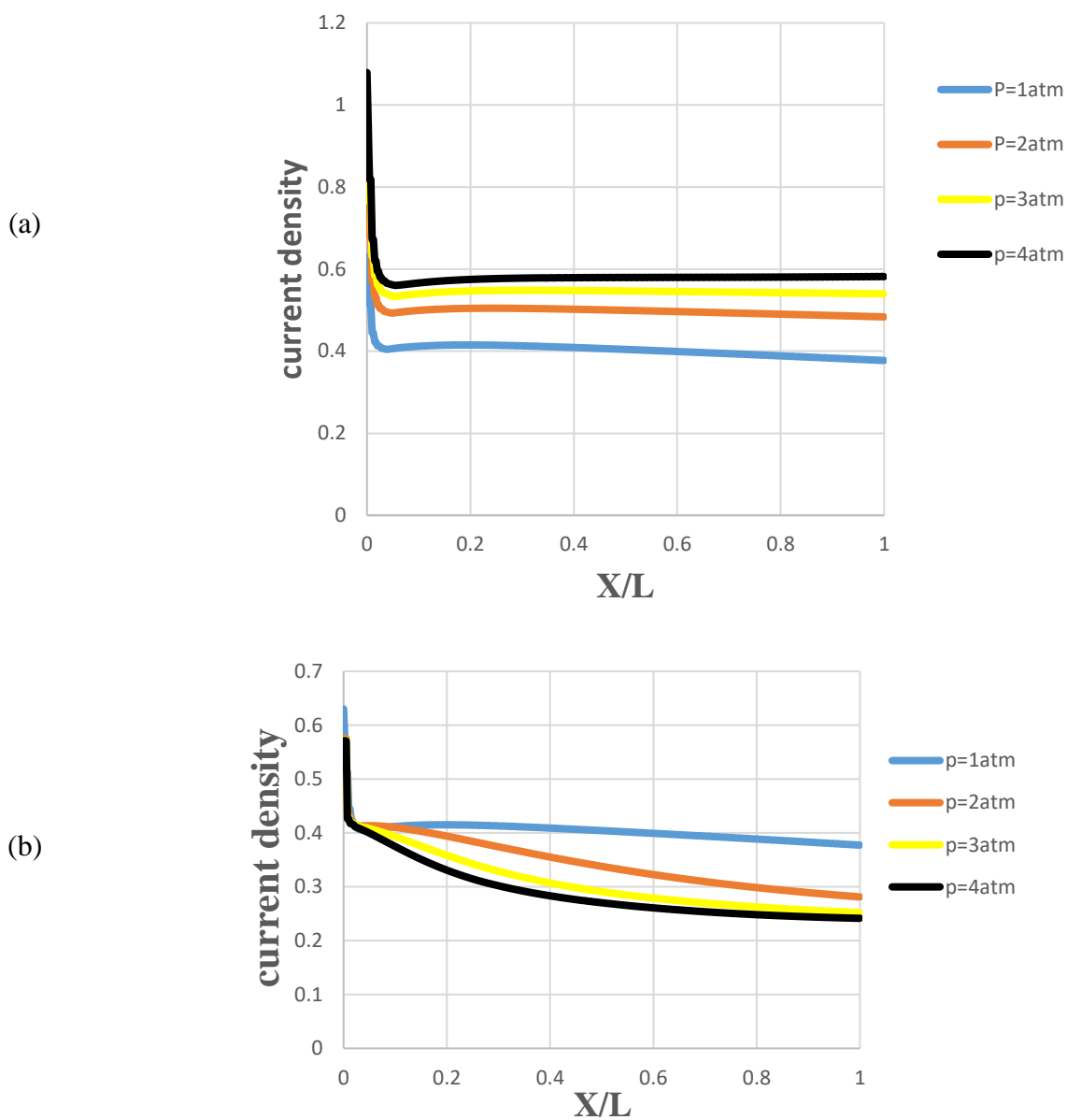
Fig3. Current density of PEM fuel cell in different pressures. (a)cathode side (b)anode side
