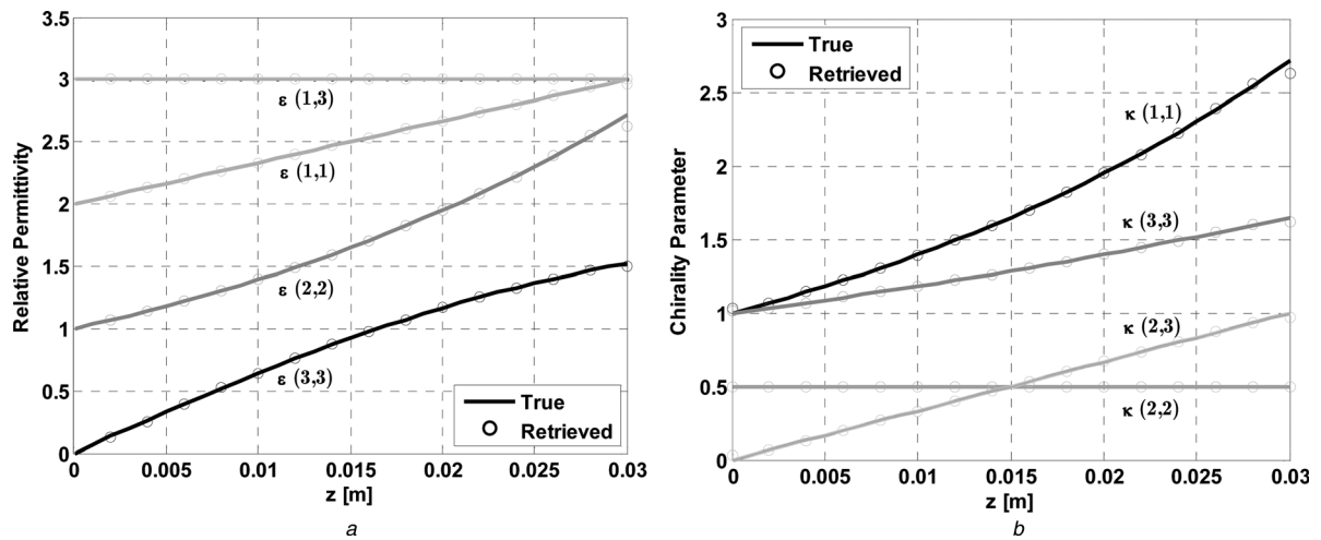
Fig. 7 Comparison of the retrieved and true unknown functions of PEC backed inhomogeneous bianisotropic slab
