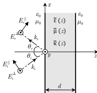
Fig. 1 Inhomogeneous bianisotropic slab exposed to an incident plane wave with TM ( E_i^{\parallel} ) or TE ( E_i^{\perp} ) polarisations
