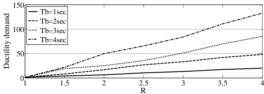
Figure 5. The effect of base isolation system stiffness on the ductility demand
