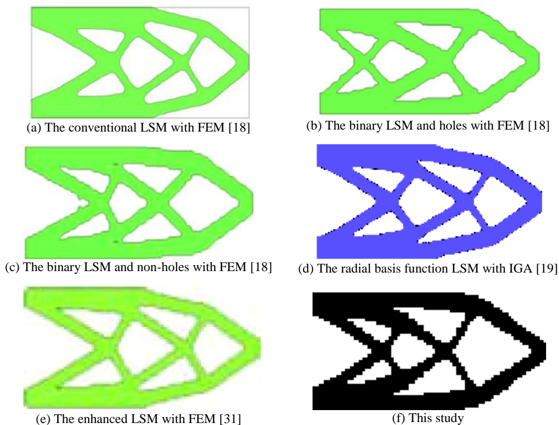
Figure 5. The comparison of the final optimal topology in this study with the other studies
