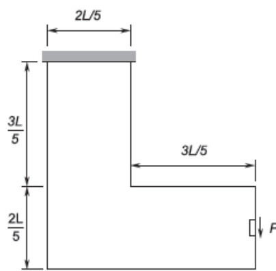
Figure 5. L-shaped structure
