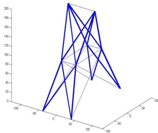
Figure 11. Optimized 25-bar truss (Model II)
