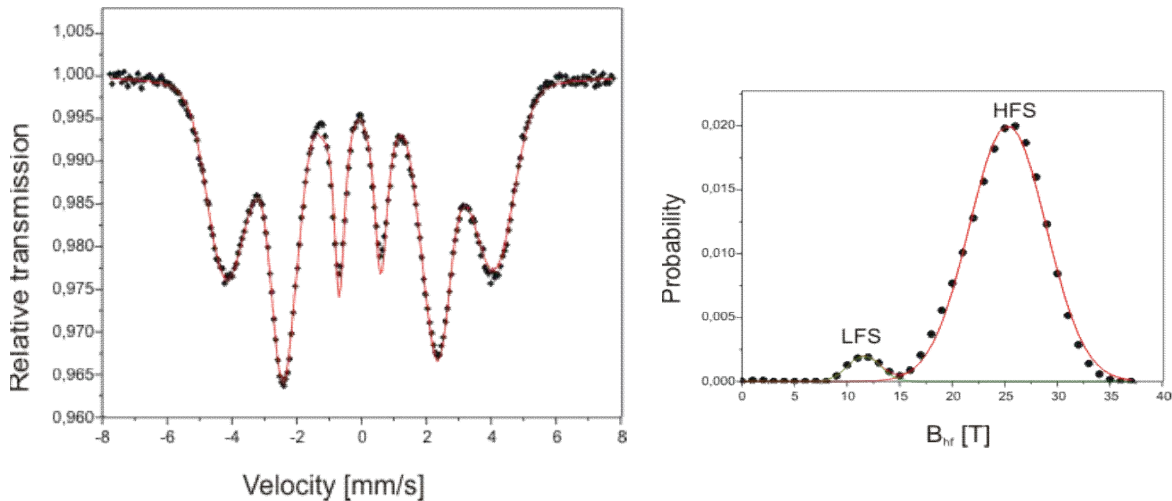
Fig. 3. Room temperature transmission Mossbauer spectrum (a) and corresponding hyperfine field distribution (b) of the as-spun Fe_{85.3}B_{11}P_3Cu_{0.7} ribbons.
