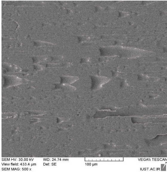
Fig. 2. SEM micrograph of the wheel side of Fe_{85.3}B_{11}P_3Cu_{0.7} ribbon, showing air pockets.
