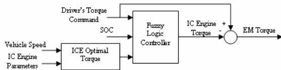
Fig. 4. Hybrid Powertrain Control Strategy.
