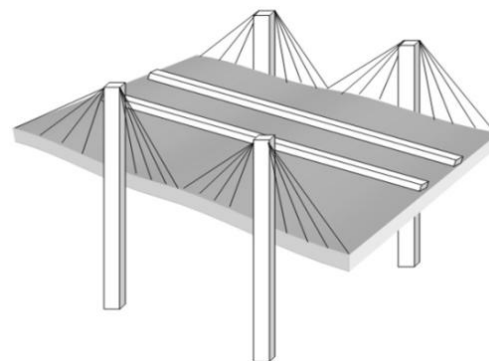
Fig. 3 3D model of the bridge
