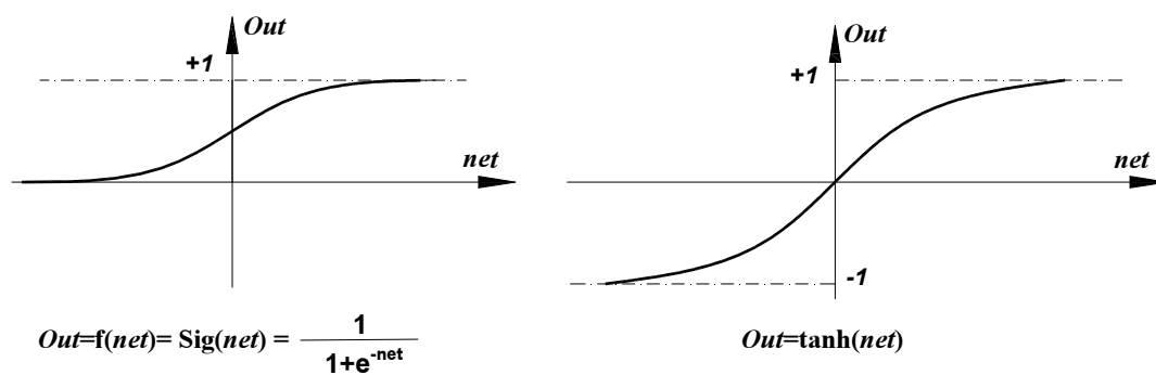
Fig. 3. Activation functions
