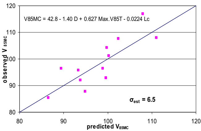
Fig. 5 (a). Comparison of observed and predicted values of V_{85MC}
