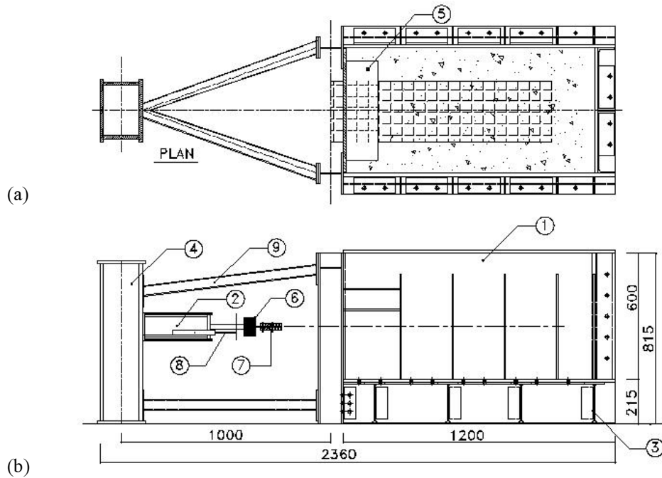
Fig. 1. (a,b) Schematic details of the pullout test apparatus.
