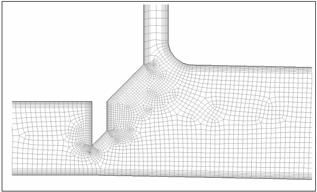
Fig. 5. Sample mesh for H=30 m, gate opening=40%
