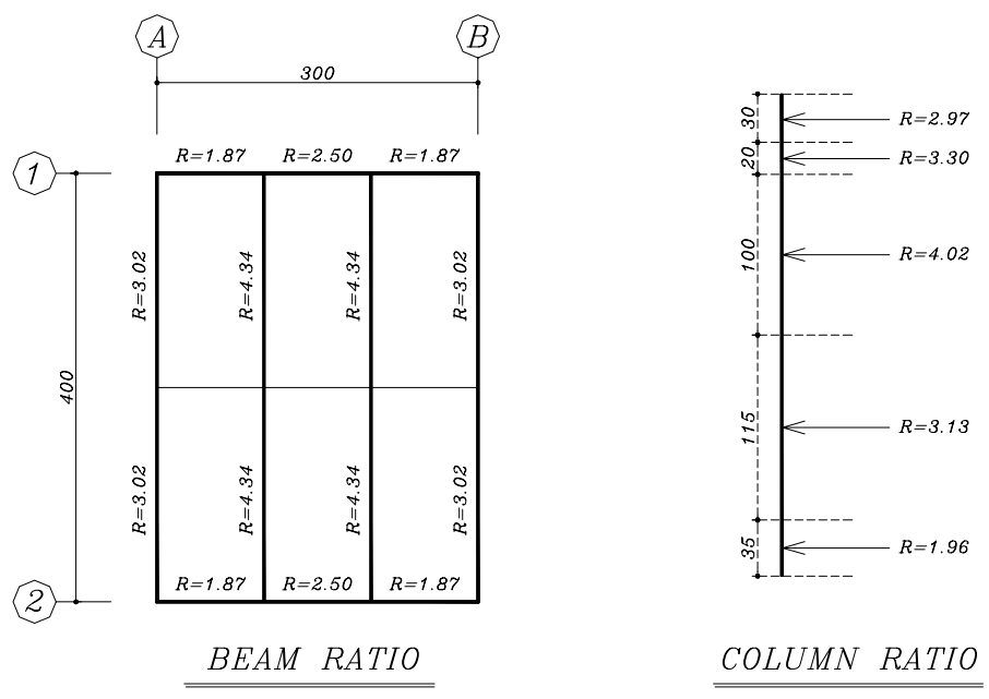
Fig.1 Stress ratios of the steel frame under uniform load ( q=2.5 \text{ ton/m}^2 )
