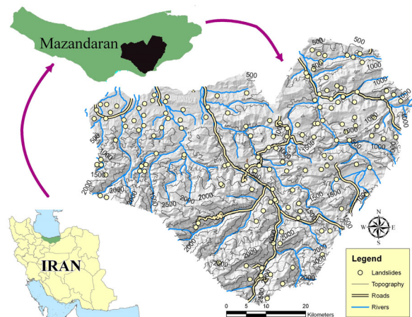
Fig. 1. Study area and landslide inventory map
