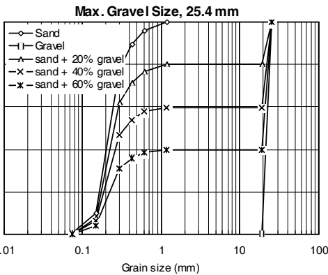
Fig.1 Gradation curves of different sand-gravel mixtures
