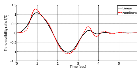
Figure 7. Wheel to body transfer ratio
